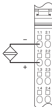
Figure 6 NAMUR input example
