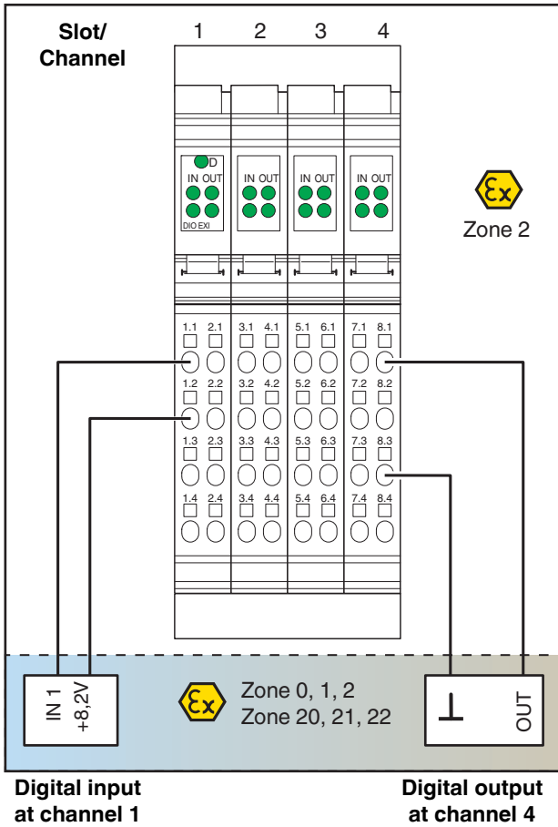
Figure 5 Connection overview
