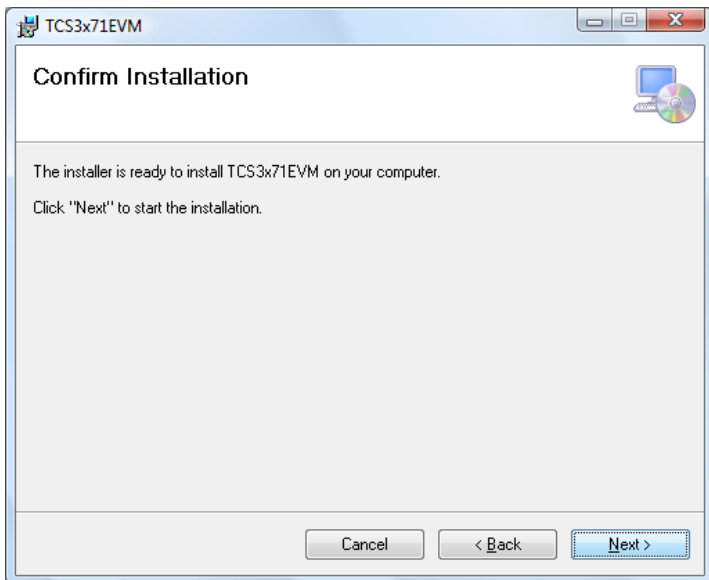
Figure 5 Confirm Installation
