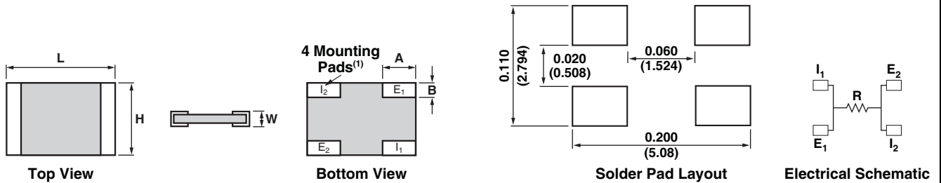
FIGURE 3 - DIMENSIONS in inches (millimeters)
