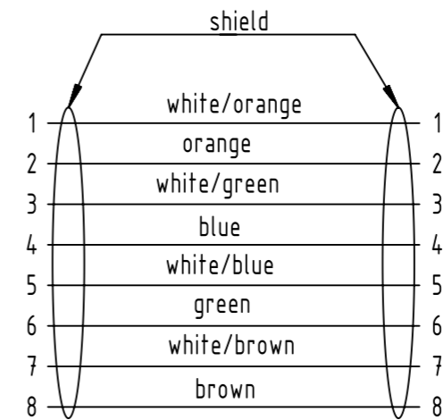
wiring plan acc.to EIA/TIA 568 B
