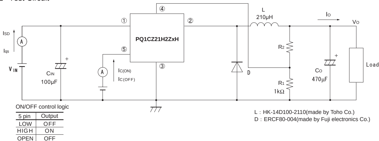
Fig.1 Test Circuit
