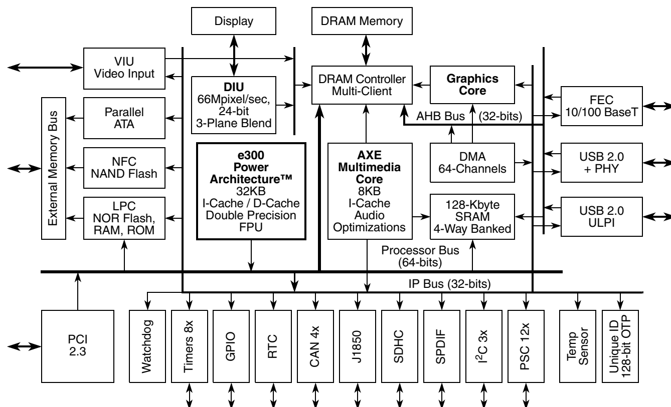
Figure 3. Multi-Core MPC5121e Block Diagram
