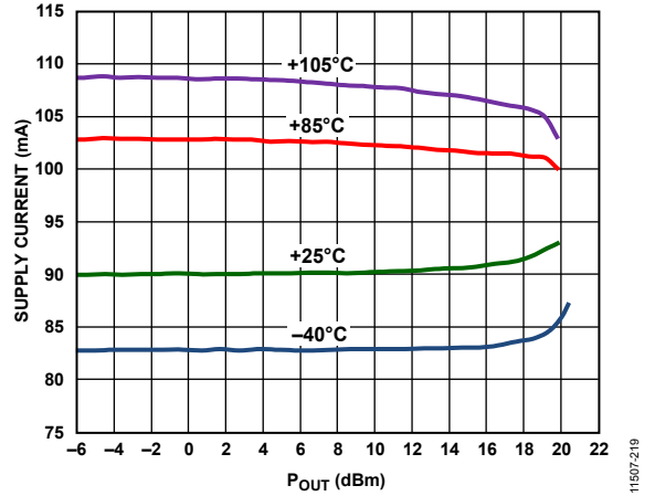
Figure 19. Supply Current vs. P_{OUT} and Temperature, V_{CC} = 5\text{ V} at 900 MHz
