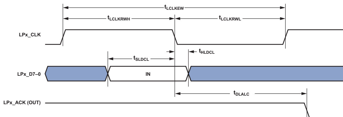
Figure 29. Link Ports—Receive
