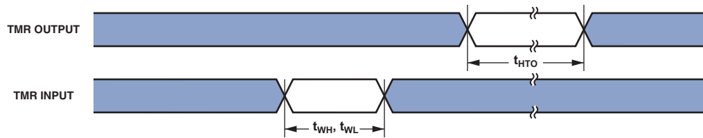
Figure 48. Timer Cycle Timing
