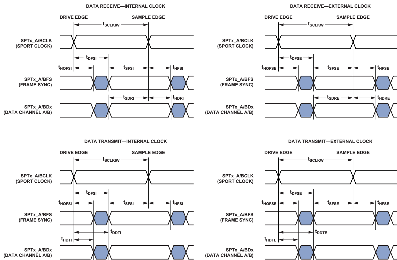
Figure 31. Serial Ports
