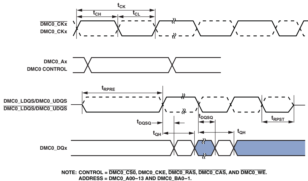
Figure 18. DDR3 SDRAM Controller Input AC Timing
