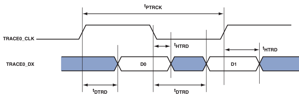
Figure 69. Trace Timing
