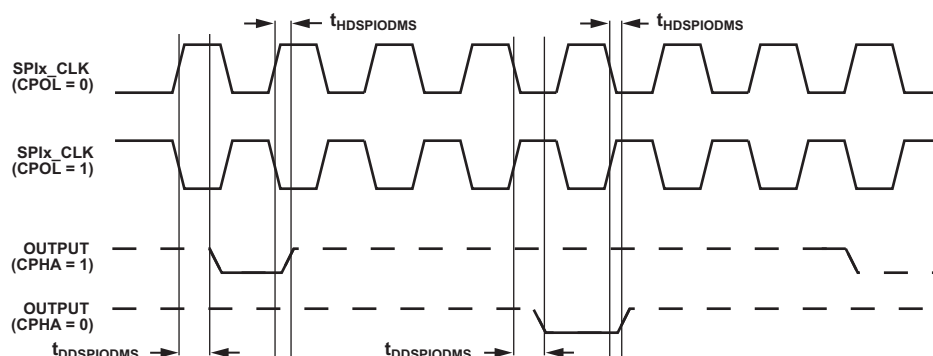
Figure 42. ODM Slave
