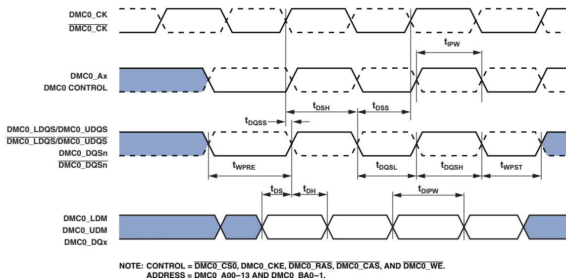
Figure 13. DDR2 SDRAM Controller Output AC Timing
