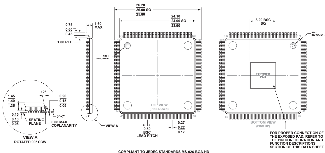
Figure 75. 176-Lead Low Profile Quad Flat Package, Exposed Pad [LQFP]
