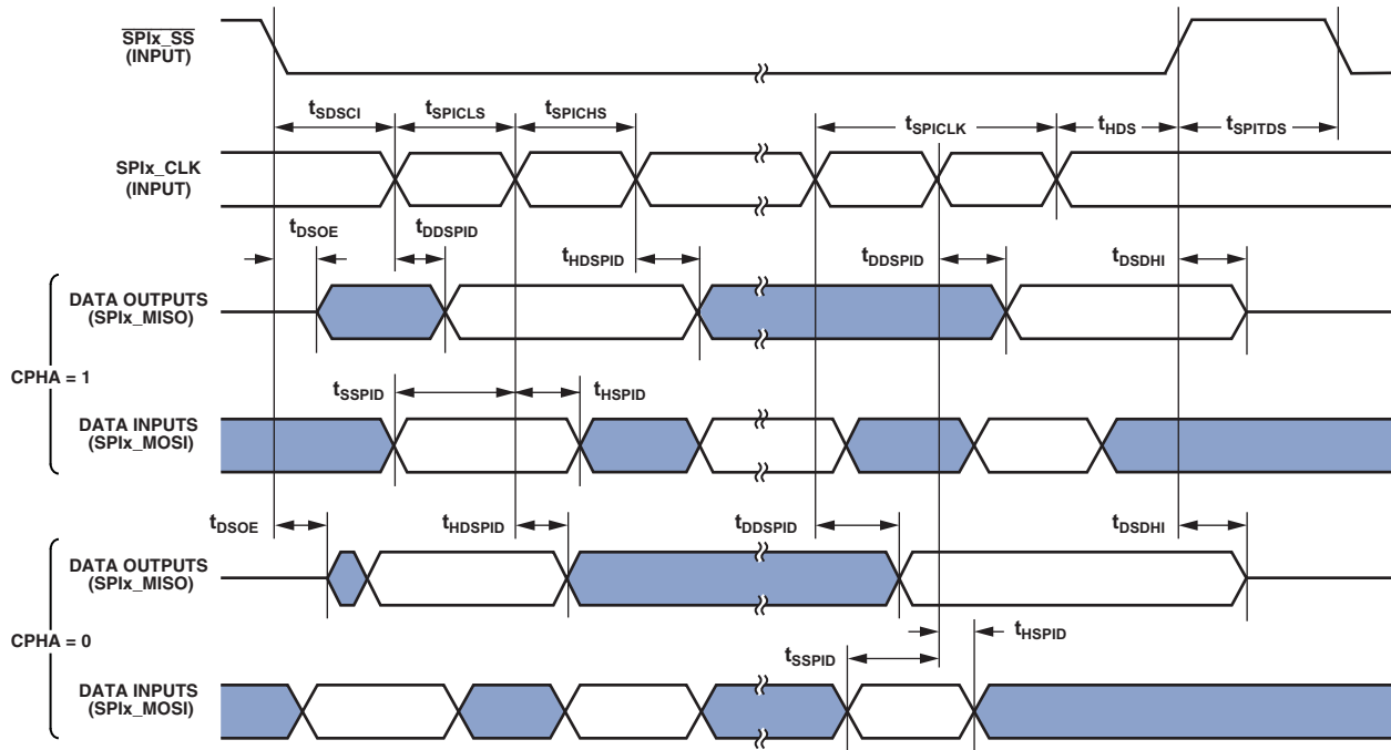
Figure 38. Serial Peripheral Interface (SPI) Port—Slave Timing
