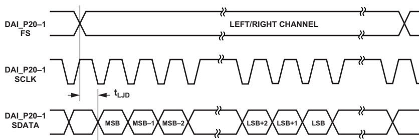
Figure 60. Left-Justified Mode
