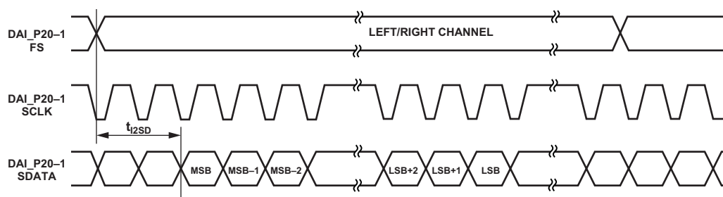
Figure 59. I 2 S-Justified Mode
