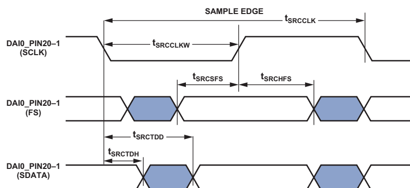
Figure 36. ASRC Serial Output Port Timing
