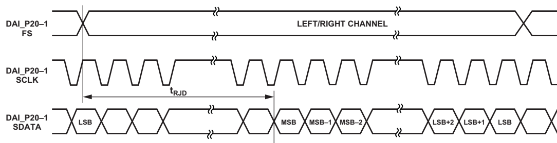
Figure 58. Right-Justified Mode
