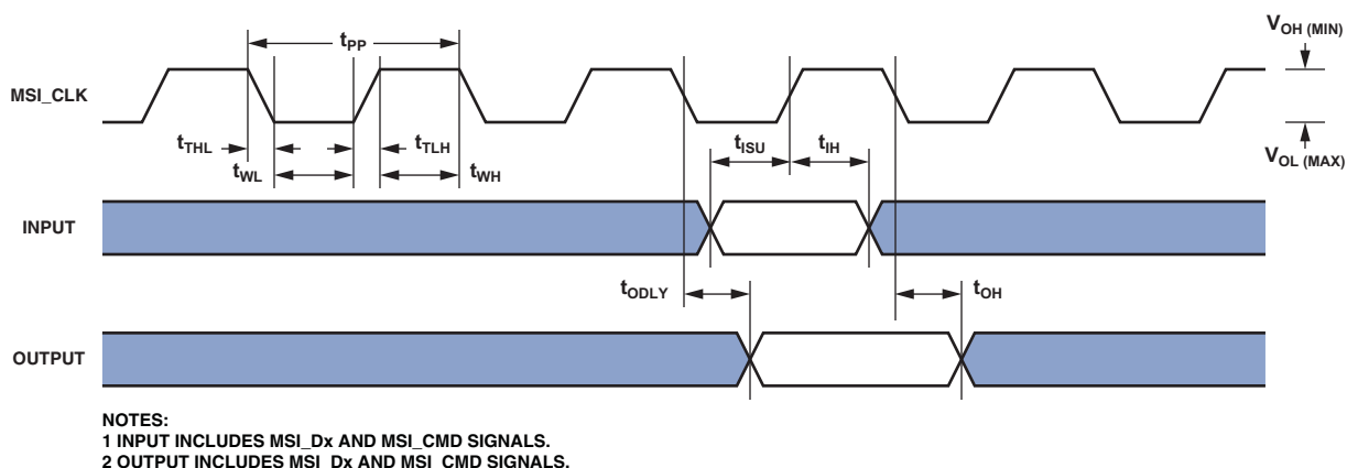
Figure 68. MSI Controller Timing
