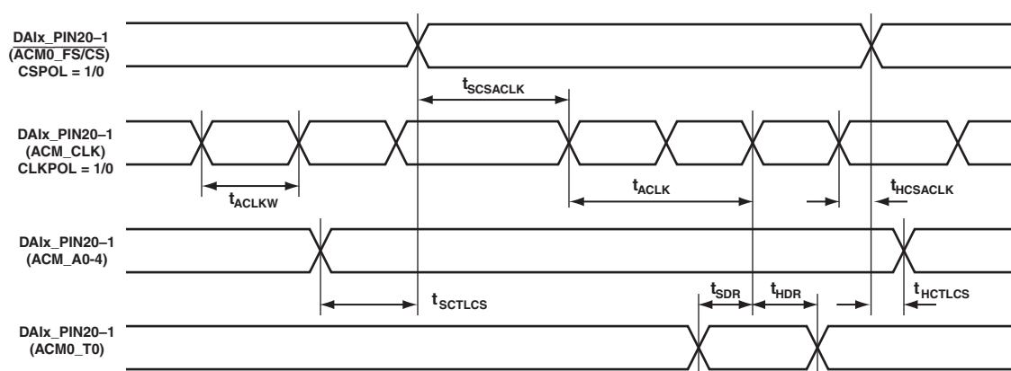
Figure 51. ACM Timing
