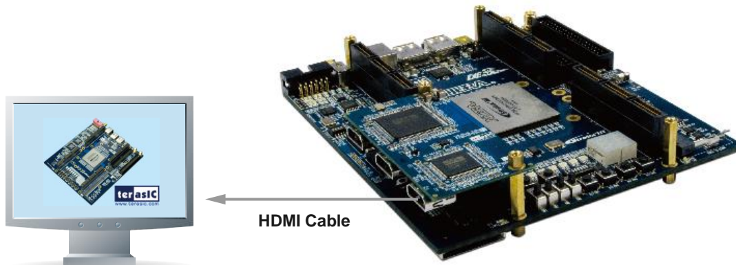
Figure 3-1 HDMI Transmission-Only Demonstration Setup
