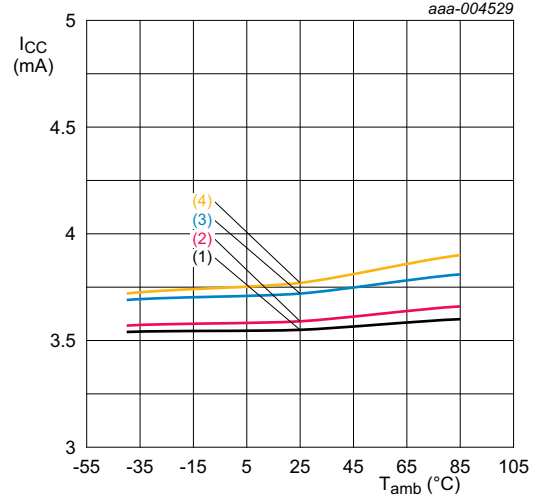
P_i = -45 dBm. (1) V_{CC} = 1.5 V (2) V_{CC} = 1.8 V (3) V_{CC} = 2.85 V (4) V_{CC} = 3.1 V
